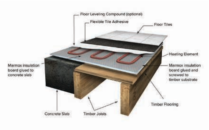
Undertile Heating with Marmox Insulation Board Installed on a Timber/Concrete Floor
