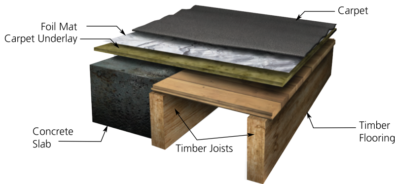
WARMUP UNDERCARPET HEATING INSTALLED ON A TIMBER/CONCRETE FLOOR
